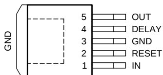
KT Package 5-Pin DDPAK/TO-263 Top View
