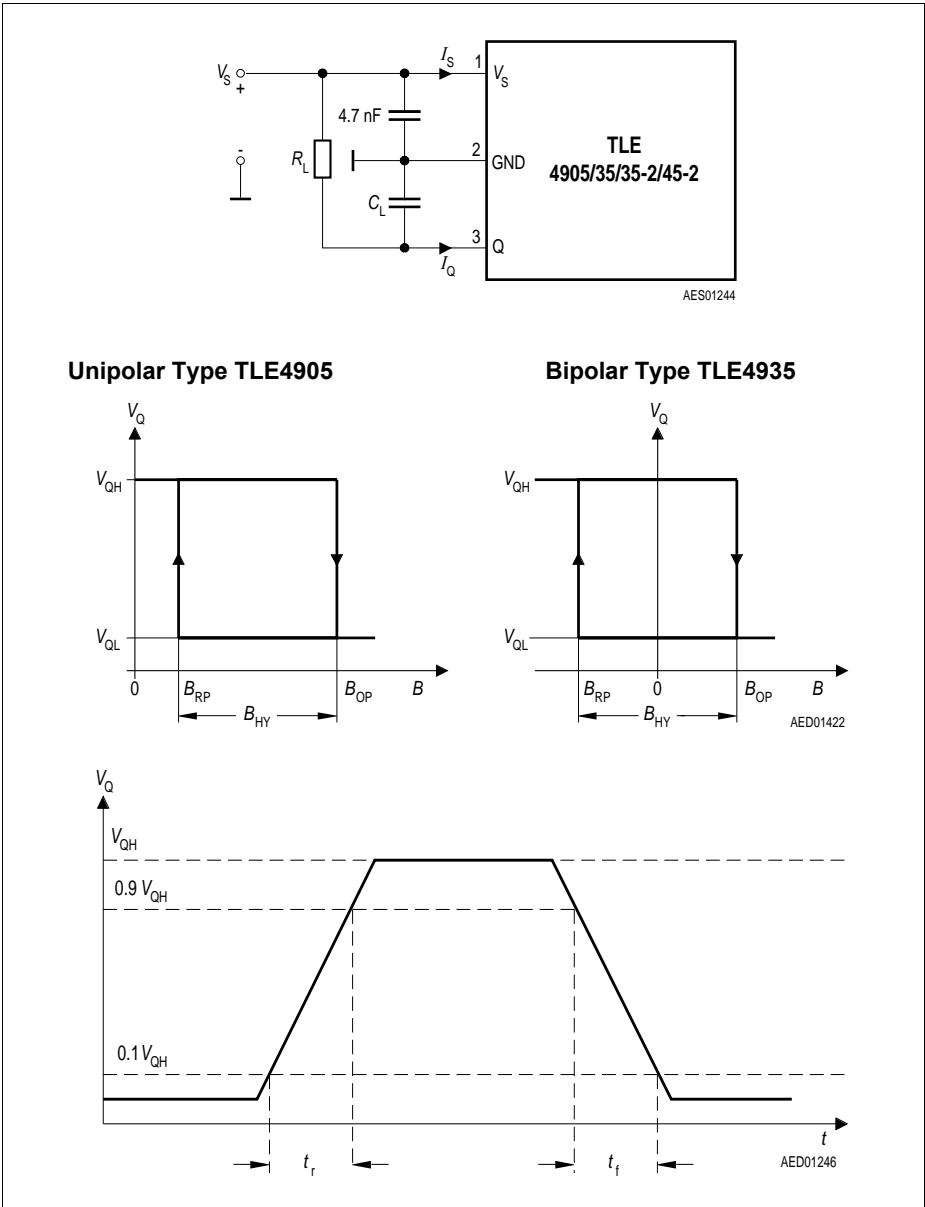
Figure 7 Test Circuit 1
