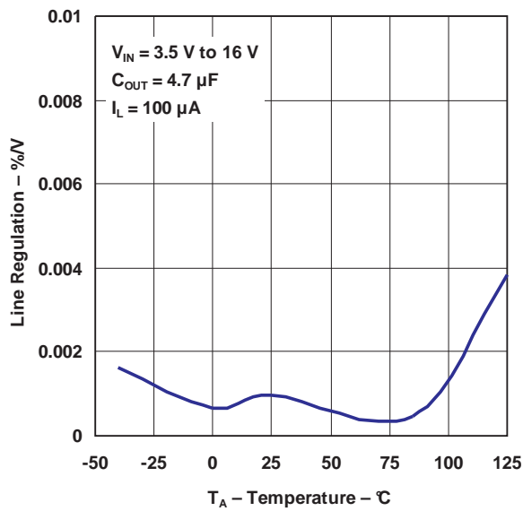
LINE REGULATION
