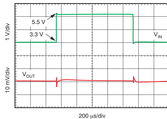
Figure 6-22. Line Transient Response
