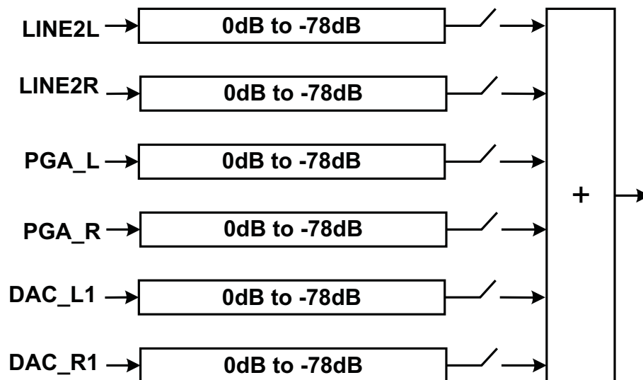
Figure 26. Detail of the Volume Control and Mixing Function Shown in Figure 21 and Figure 35
