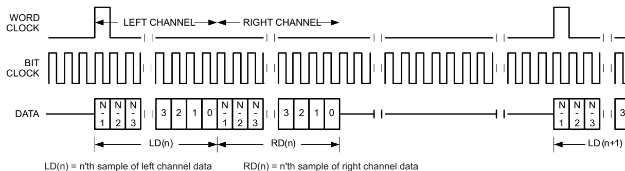
Figure 7-47. Timing Diagram for DSP Mode
