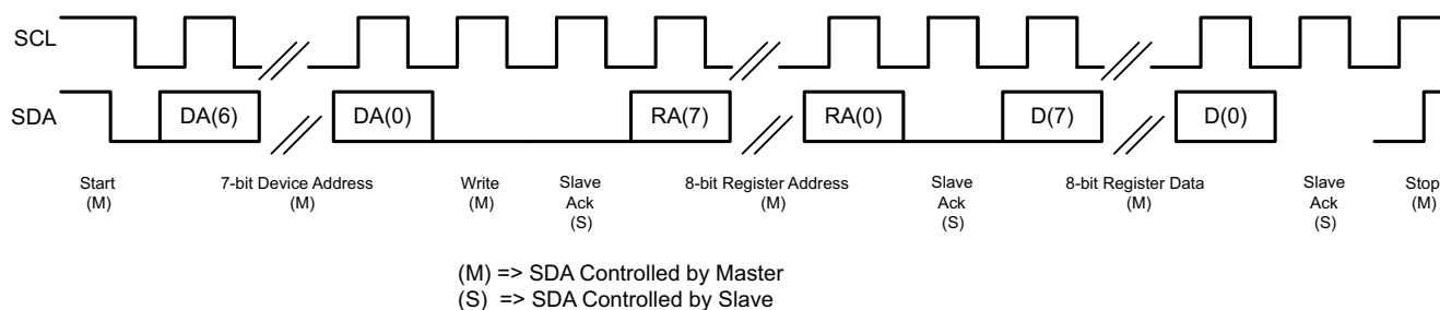
Figure 7-51. I 2 C Write
