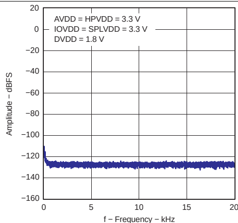
Figure 5-9. FFT – ADC Idle Channel, Single-Ended
