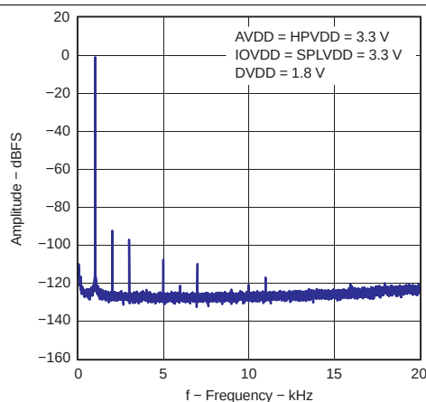
Figure 5-7. FFT – ADC Single-Ended Input
