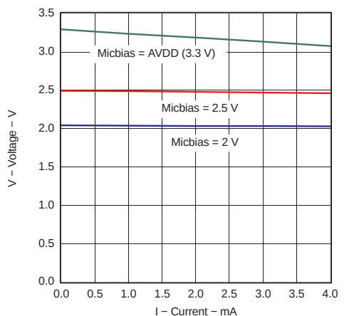
Figure 5-19. Voltage vs Current MICBIAS
