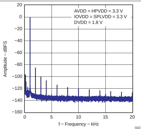
Figure 5-18. Amplitude vs Frequency FFT – Line-In Bypass to Headphone Output
