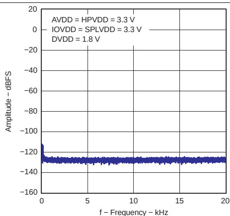
Figure 5-6. FFT – ADC Idle Channel Differential
