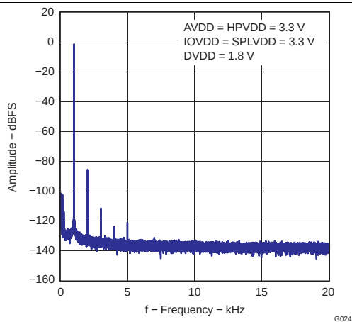
Figure 5-17. Amplitude vs Frequency FFT – Line-In Bypass to Line Output
