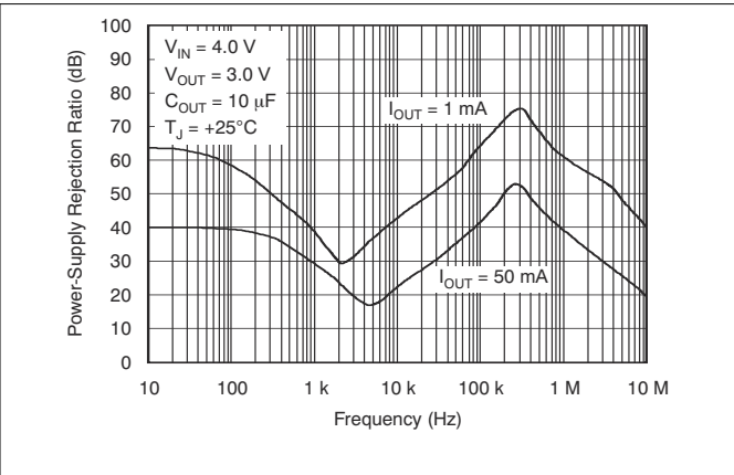
Figure 6-20. Power-Supply Ripple Rejection vs Frequency for Legacy Chip
