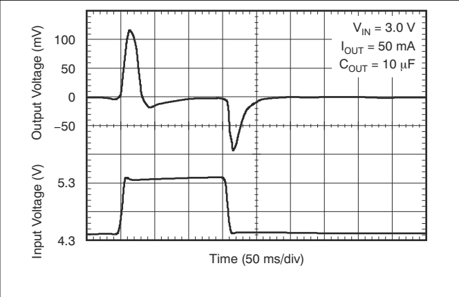
Figure 6-22. Line Transient Response for Legacy Chip
