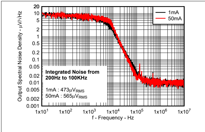
Figure 6-19. Output Spectral Noise Density vs Frequency for New Chip
