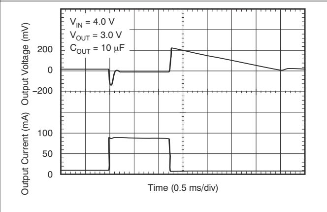
Figure 6-24. Load Transient Response for Legacy Chip
