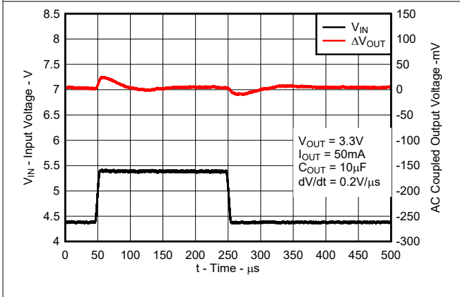
Figure 6-23. Line Transient Response for New Chip
