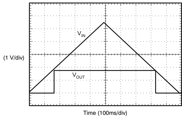
Figure 25. Power-Up and Power-Down
