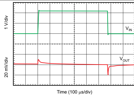
Figure 50. Line Transient Response
