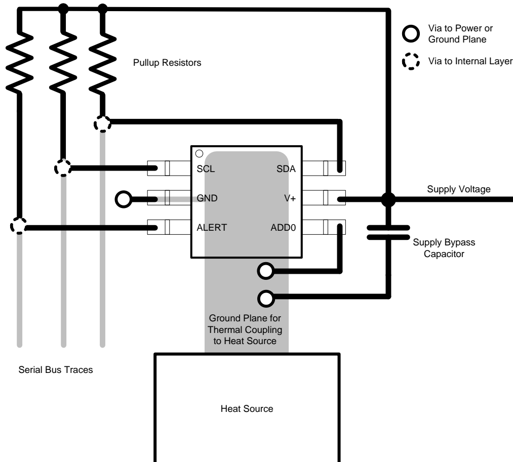
Figure 17. TMP102 Layout Example
