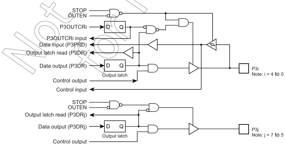
Figure 5-4 Port P3
