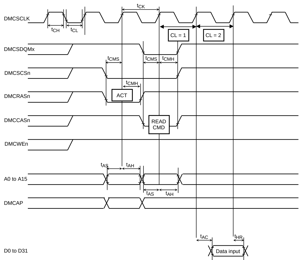
(1) SDRAM read timing (CAS latency = 2)
