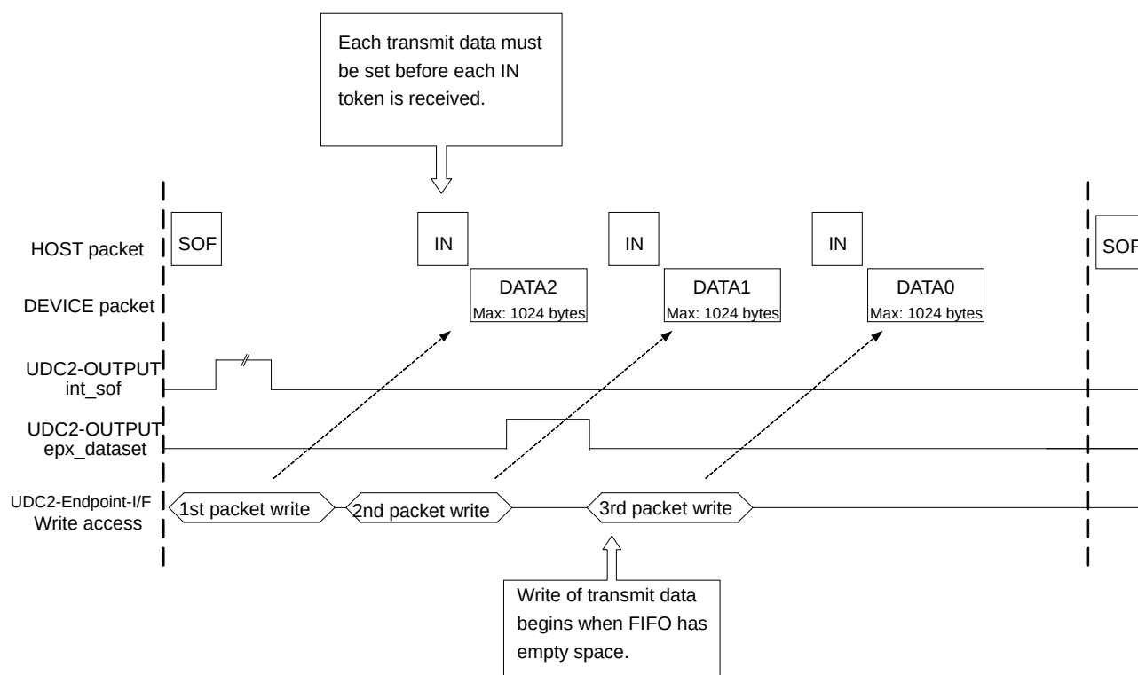
Figure 3.16.36 Isochronous IN transfers in HS mode (3 transactions)
