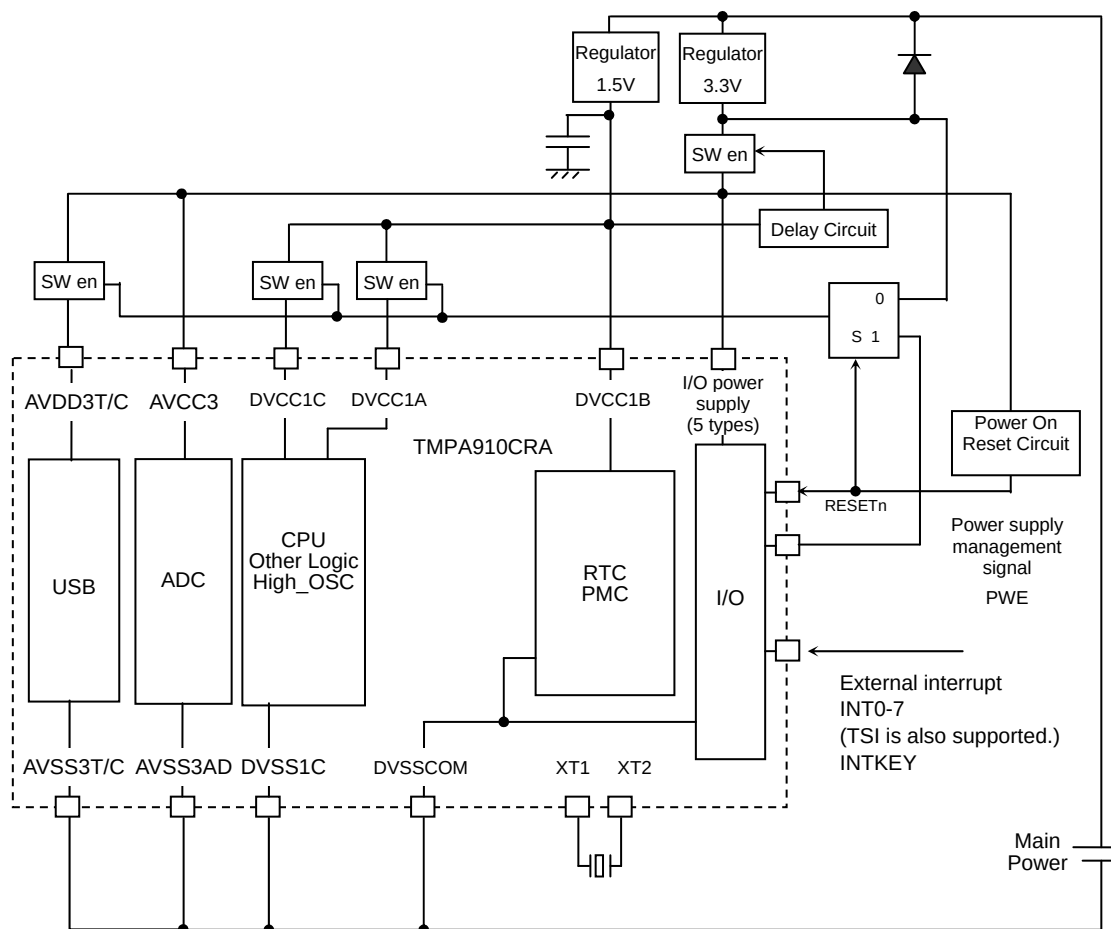
Figure 3.26.3 Power Supply System
