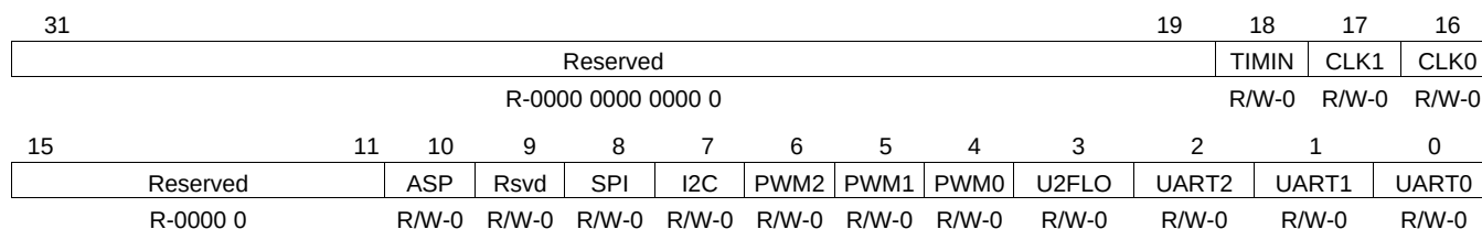
Figure 3-8. PINMUX1 Register (1)
