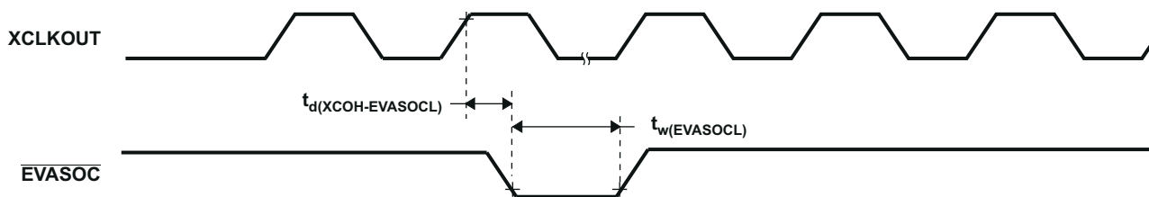
Figure 8-17. EVASOC Timing
