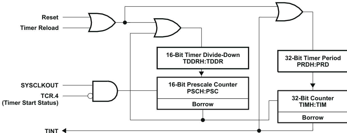
Figure 9-1. CPU-Timers
