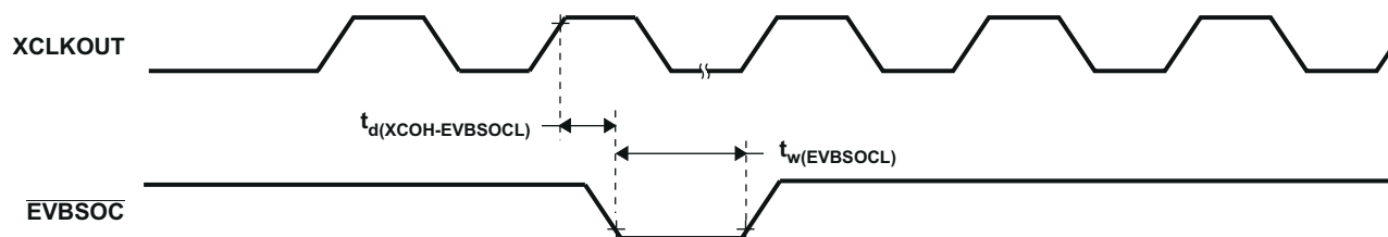
Figure 8-18. EVBSOC Timing
