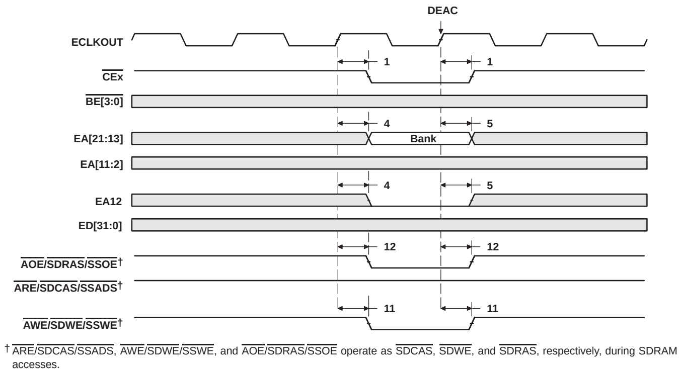
Figure 44. SDRAM DEAC Command
