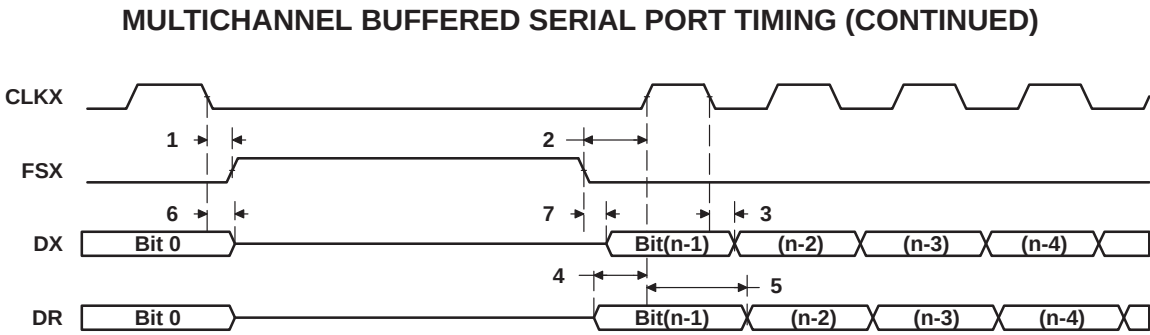
Figure 62. McBSP Timing as SPI Master or Slave: CLKSTP = 11b, CLKXP = 0
