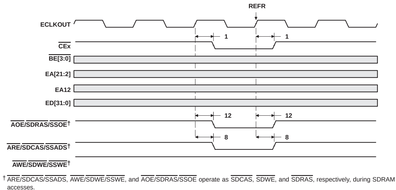
Figure 45. SDRAM REFR Command
