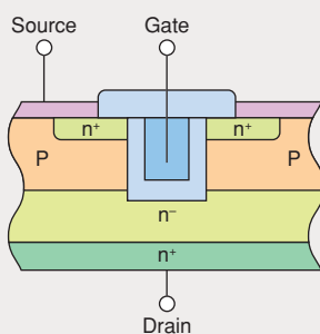
Trench Structure
