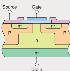
Super-Junction Structure
