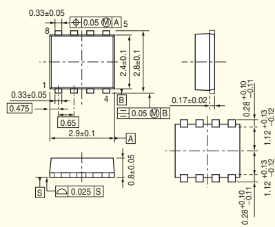
Package dimensions
