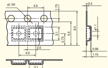
Tape dimensions
