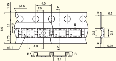
Tape dimensions
