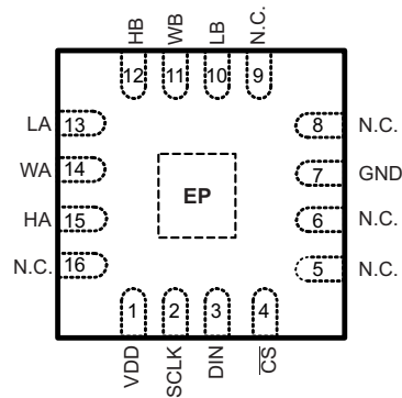
Pin Functions
