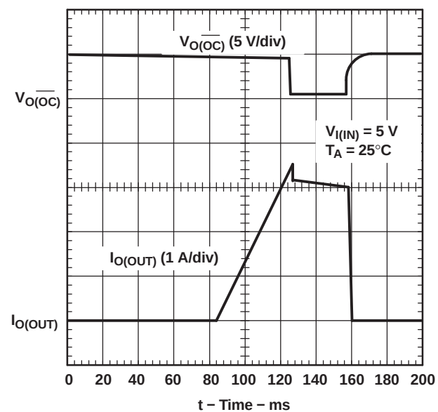
Figure 11. TPS2024, Ramped Load on Enabled Device
