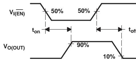
Figure 1. Test Circuit and Voltage Waveforms
