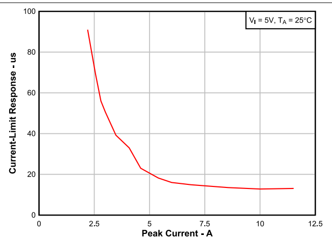
Figure 7-33. Current-Limit Response vs Peak Current
