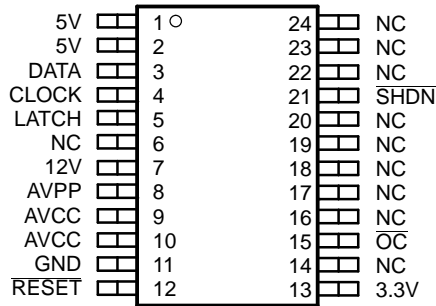
TPS2220B DB OR PWP PACKAGE (TOP VIEW)
