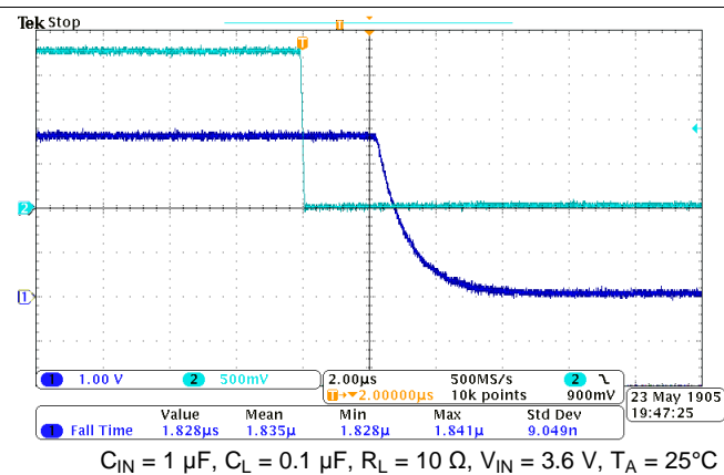
Figure 21. Turn-Off Response
