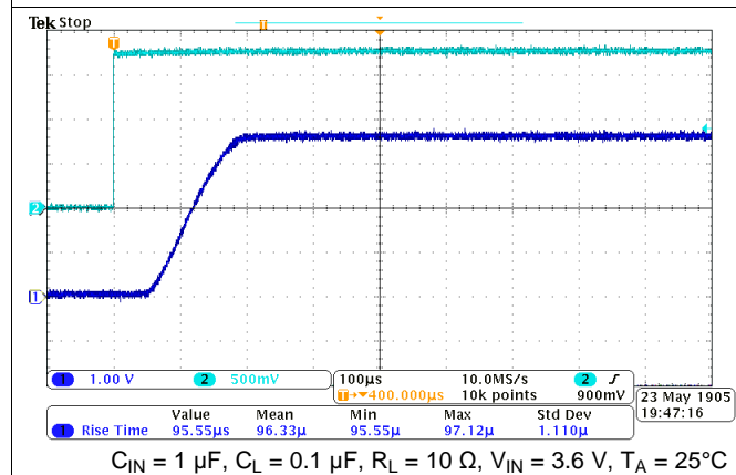
Figure 20. Turn-On Response
