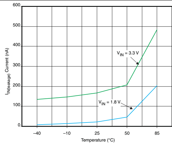
Figure 5. I_{IN(Leakage)} vs Temperature
