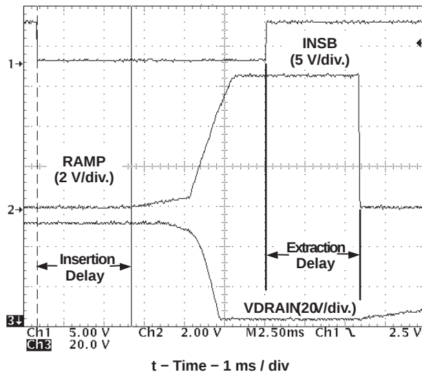
Figure 6. Insertion/Extraction Detection
