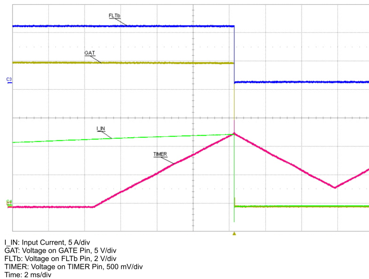
Figure 31. Circuit-Breaker Mode During Overload Condition
