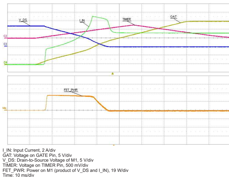
Figure 30. Computation of M_1 Power Stress During Startup
