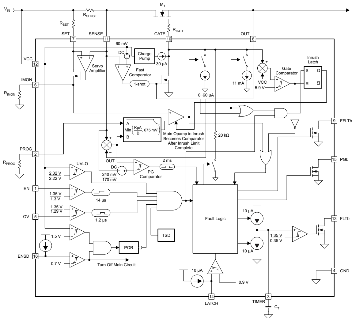
Figure 28. Block Diagram of the TPS24720
