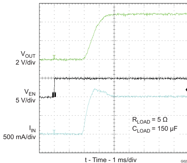
TURN-ON RESPONSE
