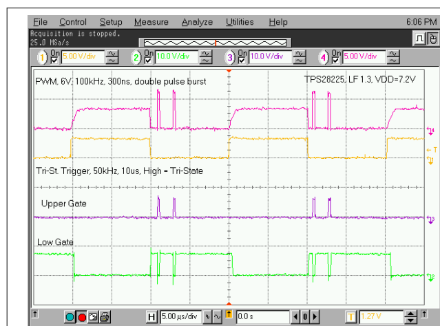
Figure 6-2. 6-V Amplitude PWM Pulse
