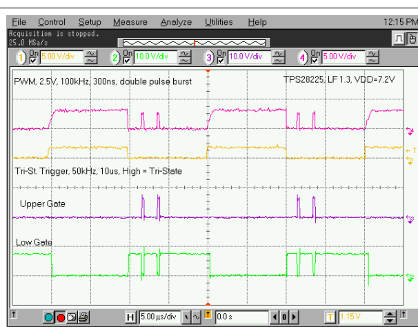
Figure 6-3. 2.5-V Amplitude PWM Pulse
