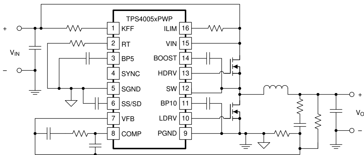
Simplified Schematic
