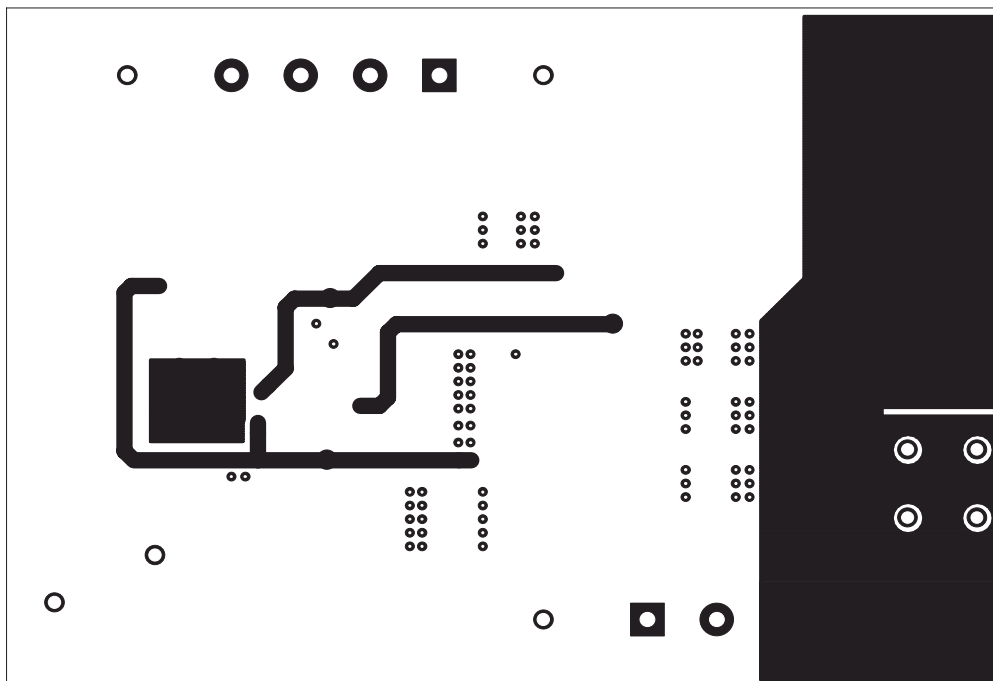
Figure 10-4. Internal Layer 2 Copper
