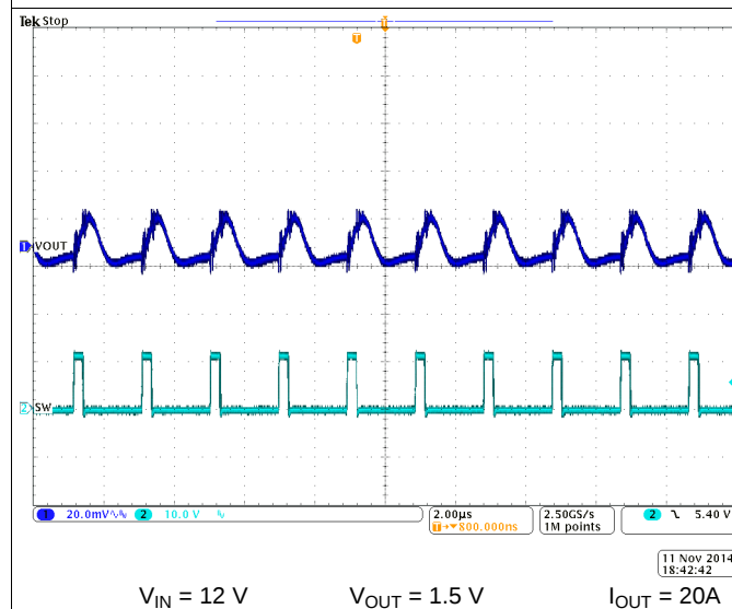
Figure 44. Output Voltage Ripple
