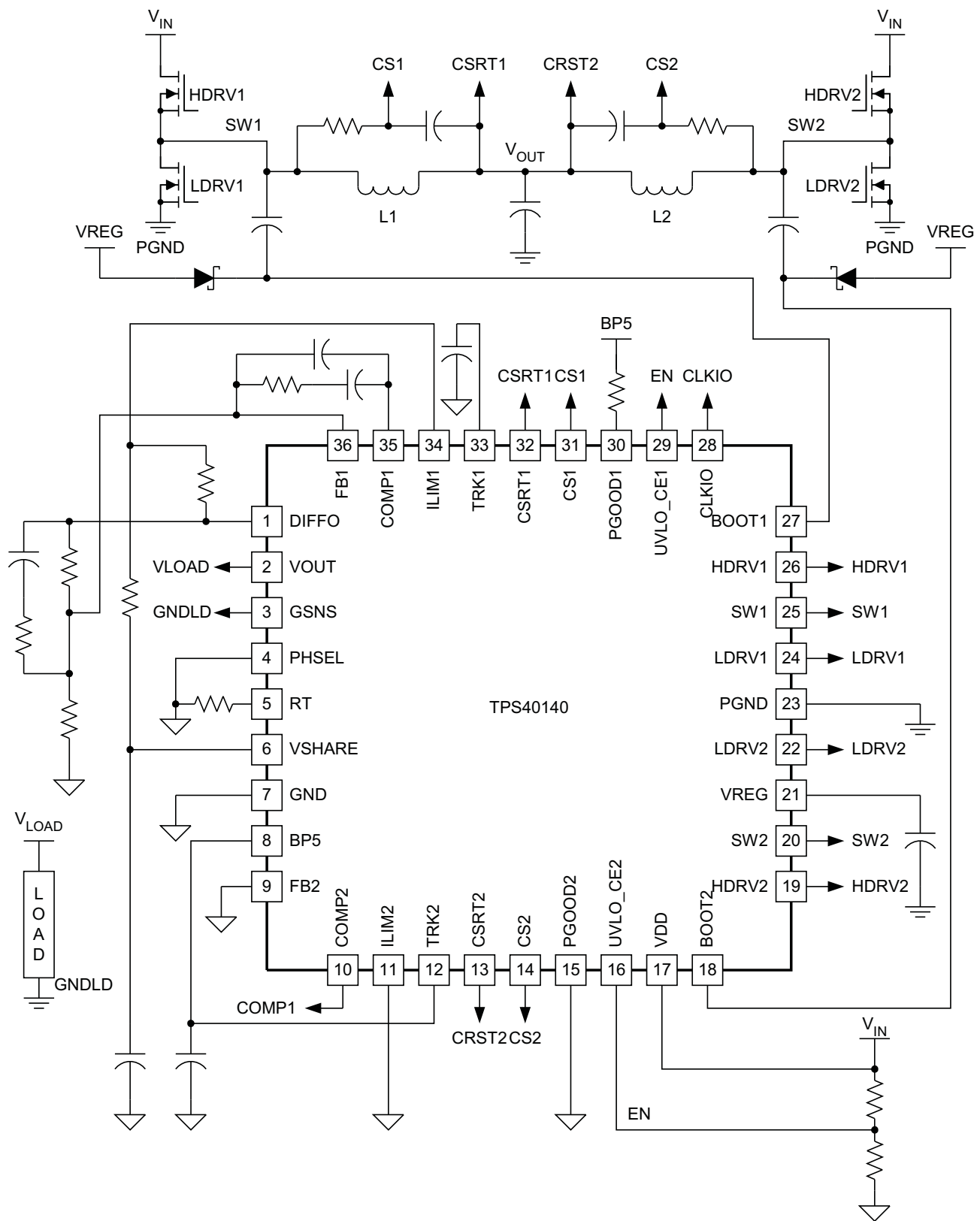
Figure 17. Typical Applications Circuit, 2-Phase Mode
