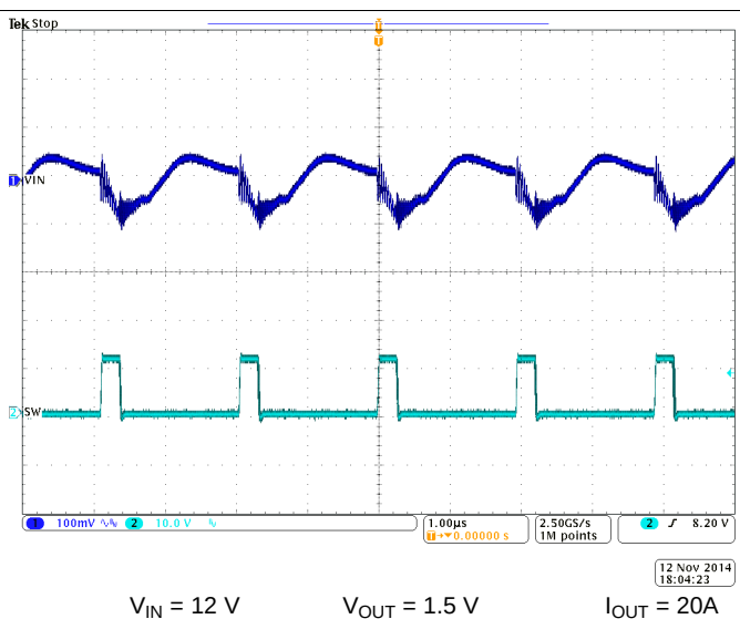
Figure 45. Input Voltage Ripple
