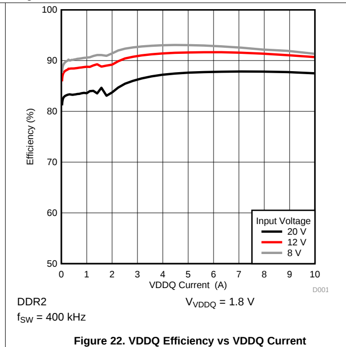
Figure 22. VDDQ Efficiency vs VDDQ Current
