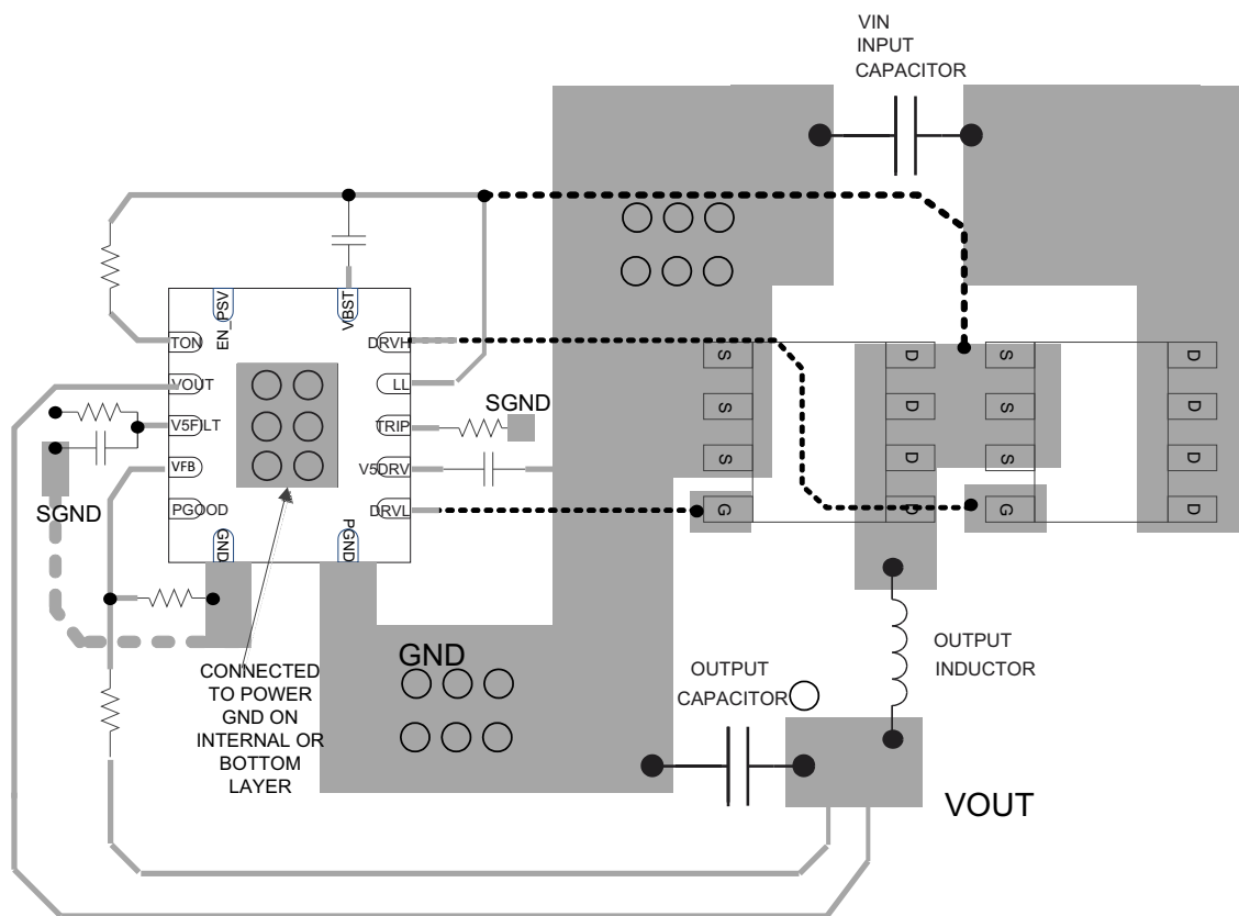
Figure 26. Layout Recommendation
