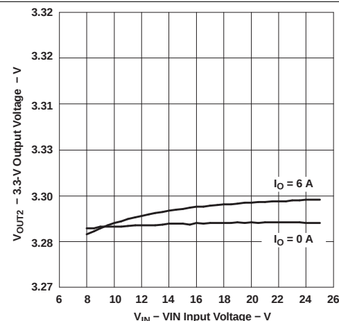
Figure 24. 3.3-V Output Voltage vs Input Voltage
