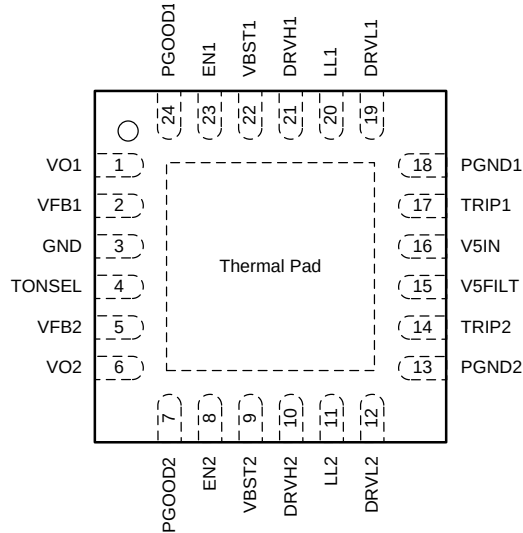
Pin Functions
