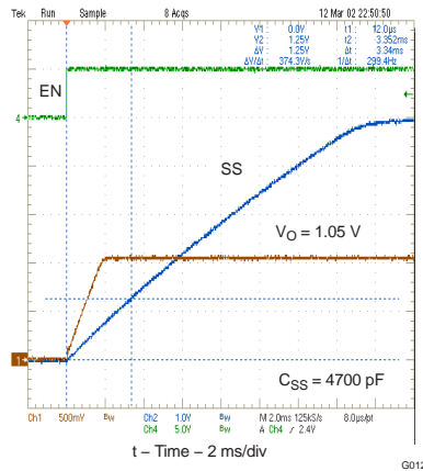
Figure 20. Startup Waveform
