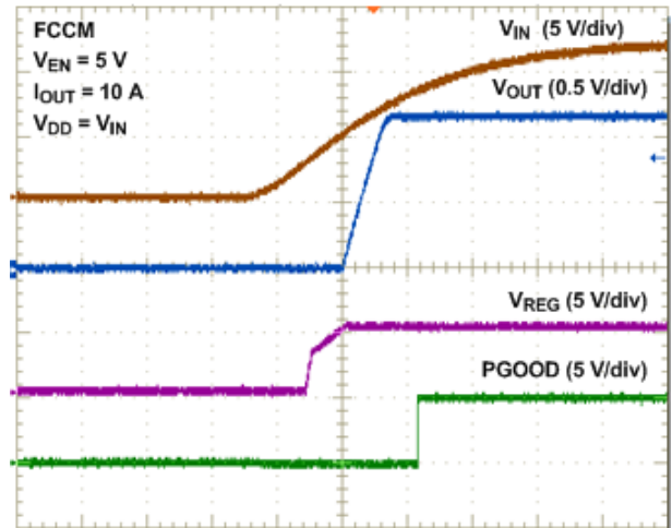
Figure 38. UVLO Start-Up
