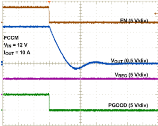
Figure 37. Shutdown
