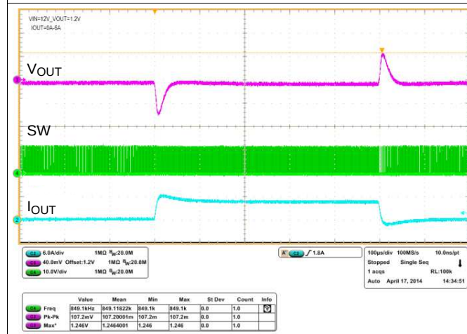
Figure 52. Full Cycle Load Transient
