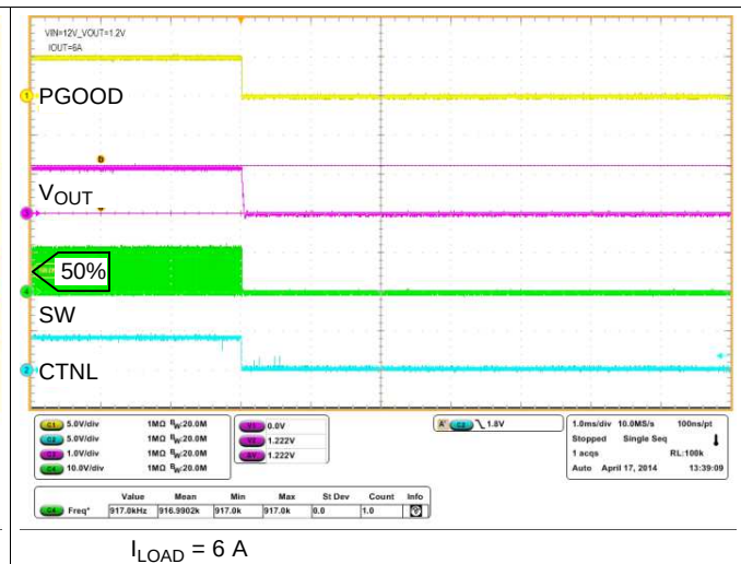
Figure 49. Shutdown Sequence
