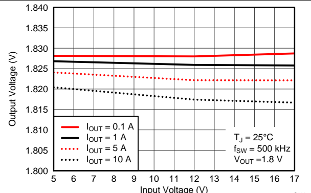
Figure 39. Line Regulation
