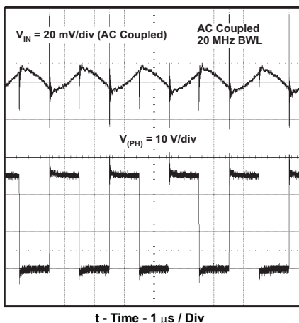
Figure 17. Output Voltage Ripple and PH Node, I_O = 1\text{ A}
