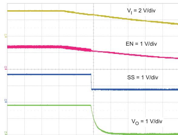
Time = 500 \mu\text{s/div} Figure 43. Power Down, V_{OUT} , V_{IN}
