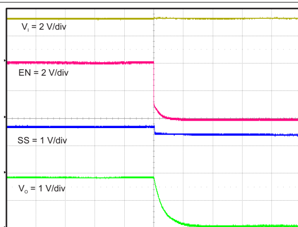
Time = 500 \mu\text{s/div} Figure 45. Power Down, V_{OUT} , EN
