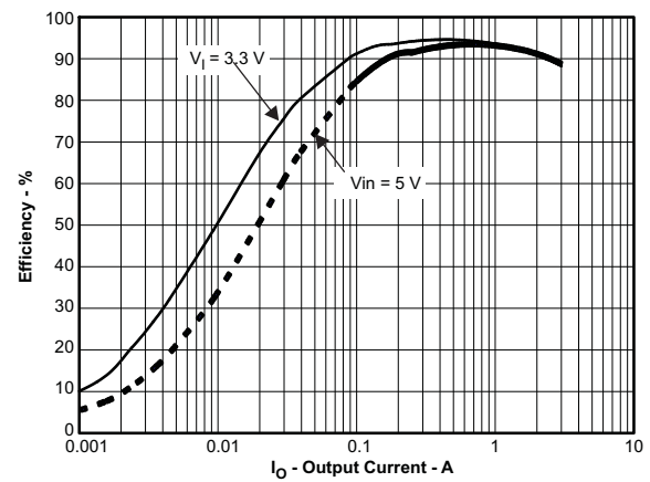
Figure 39. Efficiency versus Load Current
