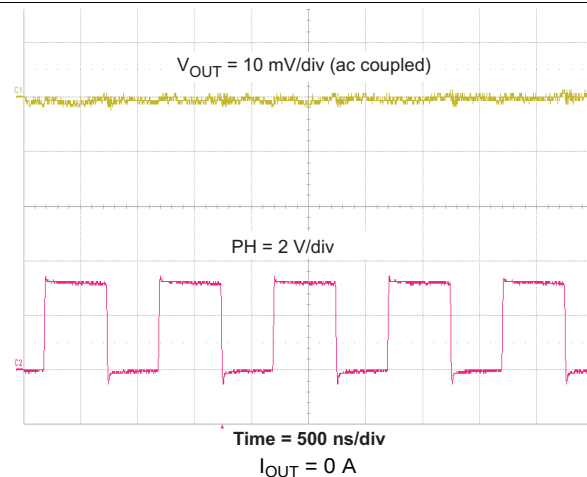
Time = 500 ns/div I_{OUT} = 0 \text{ A} Figure 47. Output Ripple
