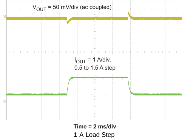
Figure 40. Transient Response
