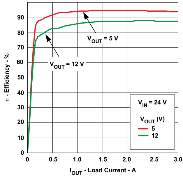
Figure 46. Efficiency vs Load Current
