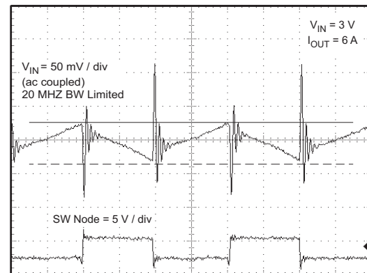
Figure 39. Input Ripple
