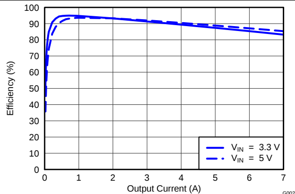
Figure 34. Efficiency vs Load Current
