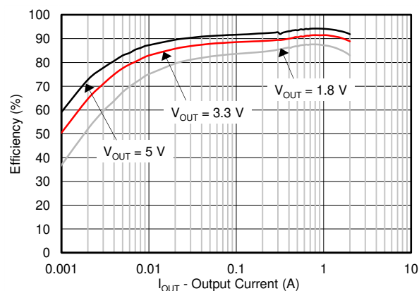
Tps562200 Efficiency
