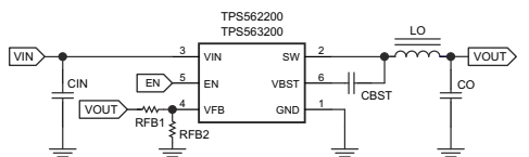
Simplified Schematic
