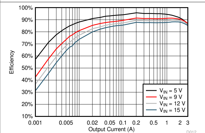
Figure 5-12. TPS563201 V_{OUT} = 3.3\text{ V} Efficiency, L = 2.2\text{ }\mu\text{H}
