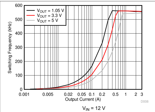
Figure 5-8. TPS563201 Switching Frequency vs Output Current
