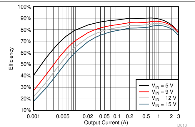
Figure 5-10. TPS563201 V_{OUT} = 1.5\text{ V} Efficiency, L = 2.2\text{ }\mu\text{H}
