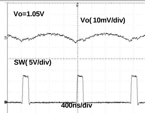
Figure 16. VOUT Ripple
