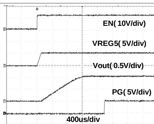
Figure 10. Slow Start
