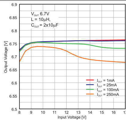
Figure 29. Output voltage vs. Input voltage, V_{OUT} = 6.7 V
