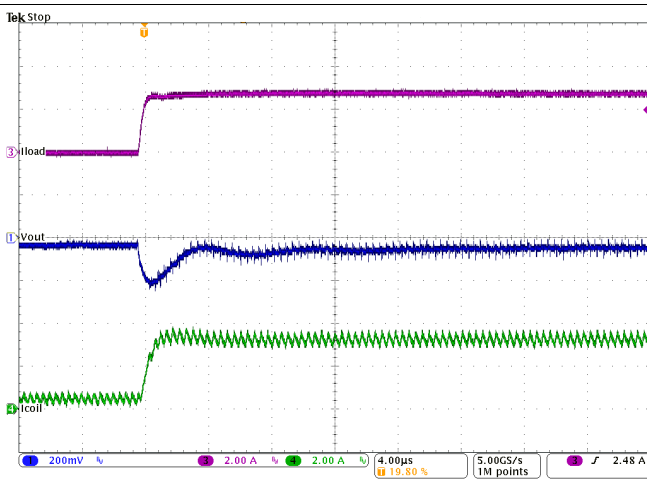
Figure 36. PWM-PSM-Transition
