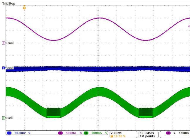
Figure 36. PWM-PSM-Transition
