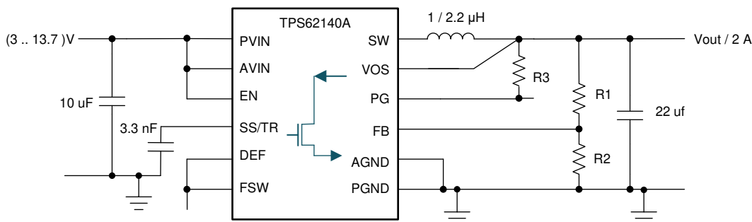
Figure 9-41. Discharge Vout through PG Pin With TPS62140A
